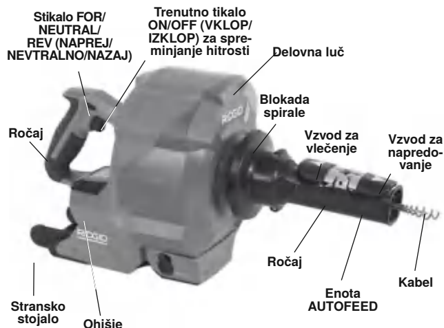
Slika 1A – RIDGID® K-46 Cordless SinkSnake
