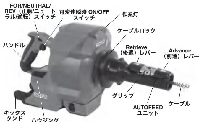
図 1A – RIDGID® K-46 Cordless SinkSnake
