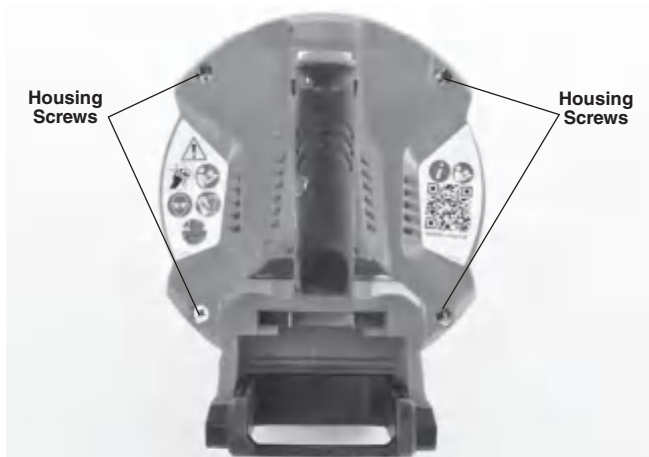
Figure 17 – Housing Screws
